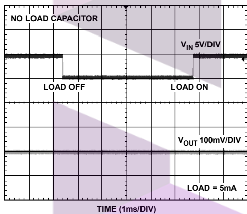
Figure 26. REF02 Load Transient Response
