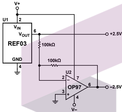
Figure 42. Bipolar Voltage Reference
