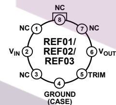
Figure 1. 8-Lead PDIP (P-Suffix), 8-Lead Cerdip (Z-Suffix), 8-Lead SOIC (S-Suffix)
